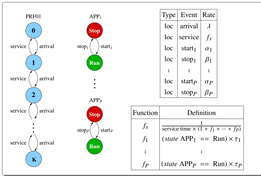
Figure 4: SAN model proposed for Phase I.
