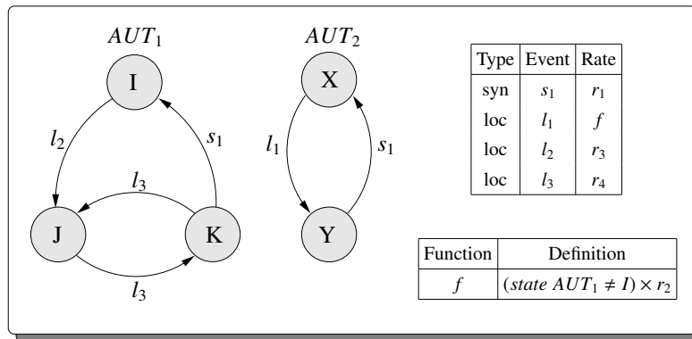
Figure 2: SAN example having local and synchronizing events with constant and functional rates.
