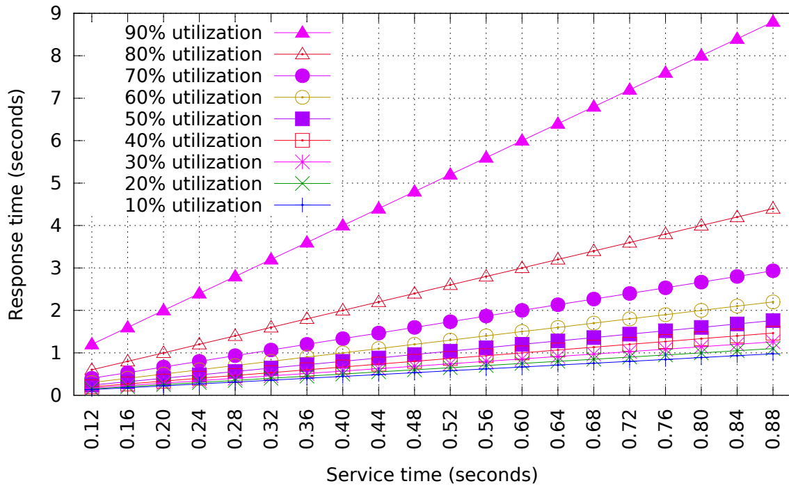
Figure 3: Maximum Response Time according to utilization choice for Phase II.
