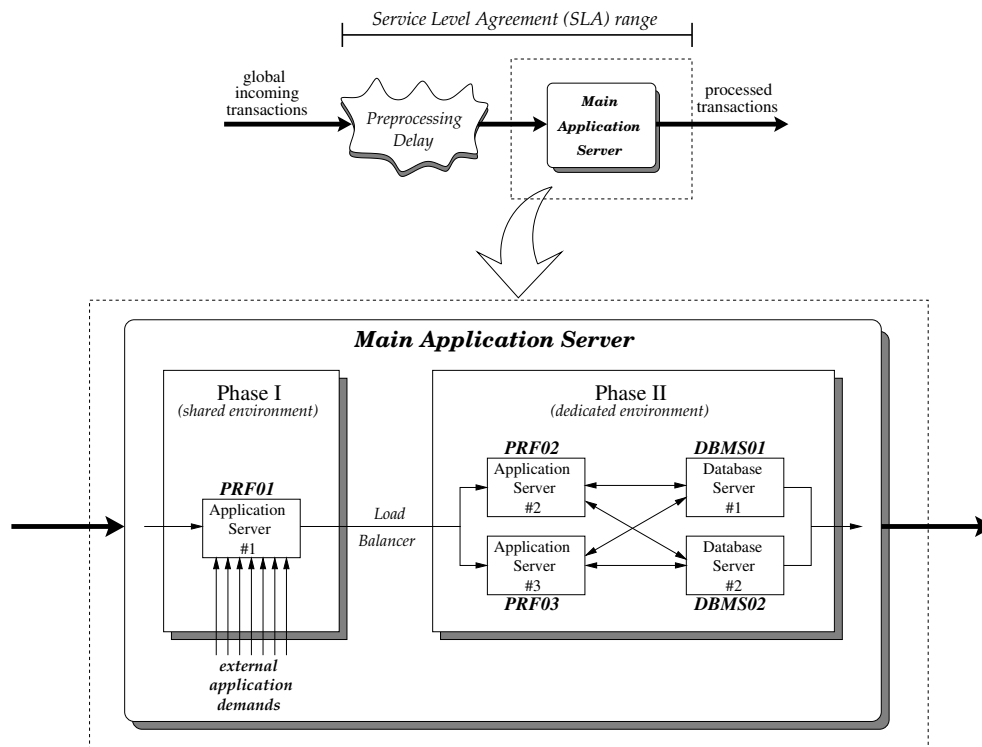
Figure 1: Main architecture and details of the testing environment.
